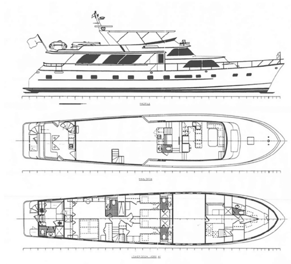
General arrangement
