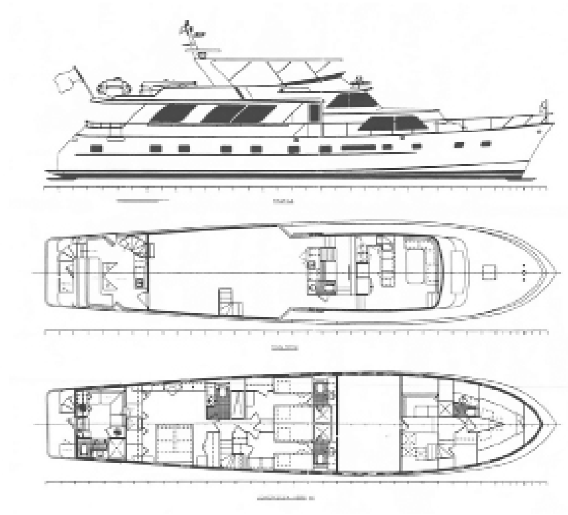
General arrangement
